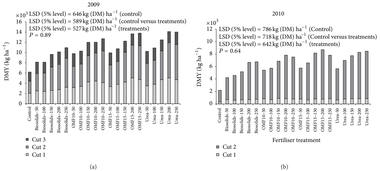
FIGURE 2: Dry matter yield (DMY) of the grass crop as affected by the fertiliser treatment in 2009 (a) and 2010 (b). The x -axis shows the fertiliser type followed by the corresponding N application rate in kg per ha. Use n = 4 (control) and n = 3 (treatments) except when N = 250 \text{ kg ha}^{-1} , n = 2 .
