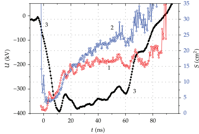
Figure 7: Change in cathode emitting surface during electron current generation, for cathodes of diameter (1) 45 mm, S = 16 \text{ cm}^2 and (2) 60 mm, S = 28 \text{ cm}^2 . (3) represents a waveform of voltage.
