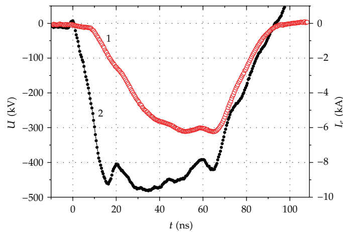
Figure 4: Waveforms of (1) electron current and (2) voltage.
