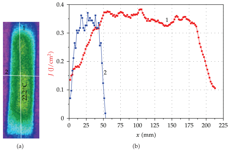
Figure 11: Thermal imprint (a) and ion beam energy density distribution at the target (b) in the vertical section (1) and horizontal section (2).
