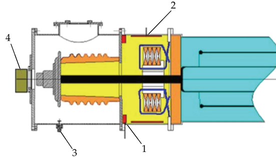
Figure 1: Diagnostic equipment of the pulsed electron accelerator: (1) Rogowski coil, (2) capacitive voltage divider, (3) differential voltage divider, and (4) Faraday cup.
