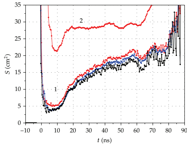
Figure 8: Change in cathode emitting surface during the generation of a pulse of current for a 60 mm diameter cathode made of (1) graphite and (2) carbon fabric.
