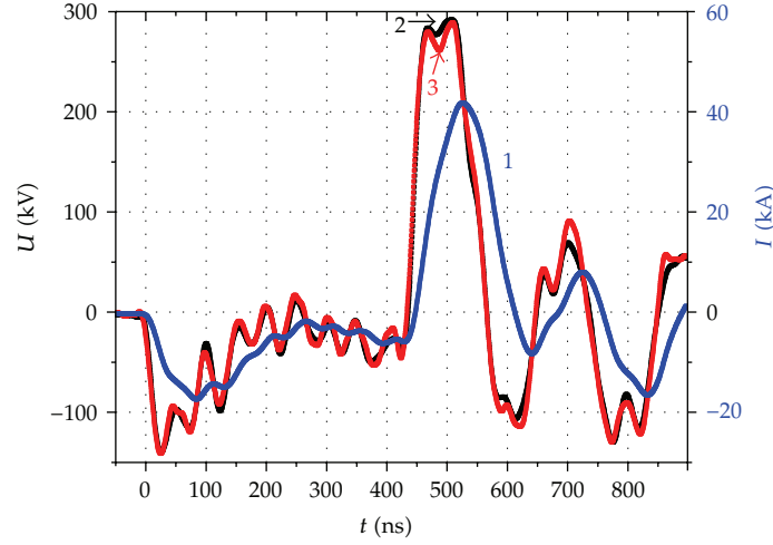
Figure 9: Waveforms of (1) current, (2) experimental, and (3) calculated voltage.
