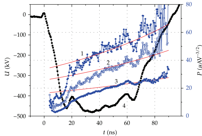
Figure 5: Experimental (dots) and calculated (solid line) values of the perveance of the planar diode with a graphite cathode with a diameter of 45 mm and gap of (1) 11, (2) 12.5, and (3) 14 mm. (4) represents a waveform of voltage.
