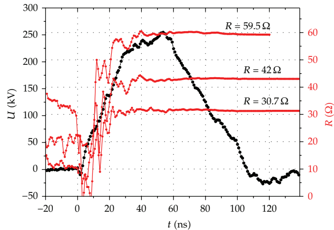
Figure 2: TEU-500 accelerator calibration using various load resistors.
