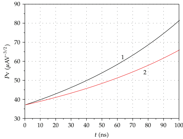
Figure 3: Calculated time-dependent change in perveance of the planar diode, taking into account (1) both the reduction of the A-K gap and increase in cathode area (radial plasma expansion); (2) only the reduction of the A-K gap.
