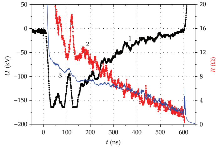
Figure 10: Waveforms of (1) voltage, (2) experimental, and (3) calculated impedance values.
