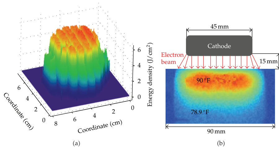
Figure 6: Distribution of the energy density over the cross-section of electron beam, measured by a radiochromic film, (a) and temperature distribution along the depth of a foam sample, measured by infrared camera (b).
