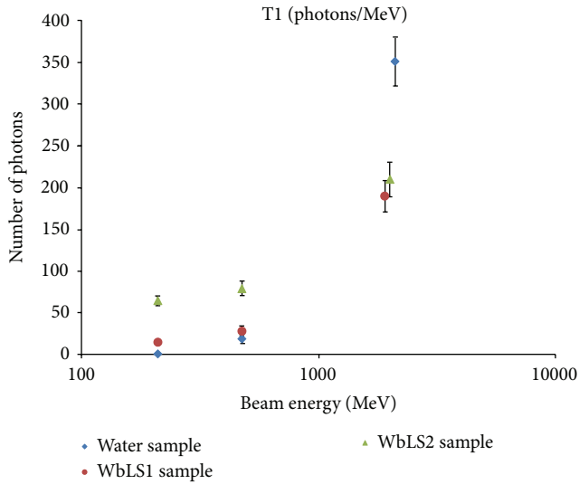
FIGURE 14: The light yield in photons/MeV for T1. At 2 GeV beam energy; some points are offset for clarity.
