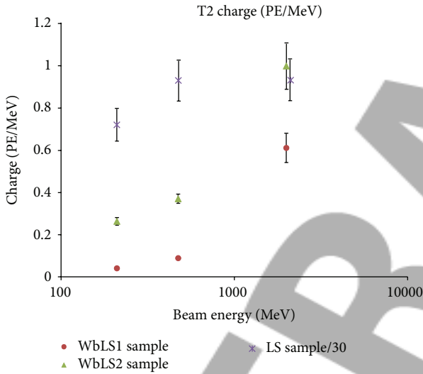
FIGURE 11: The light yield in PE/MeV for T2. At 2 GeV beam energy, some points are offset for clarity.
