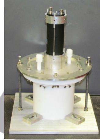
FIGURE 2: PTFE tub detector with a PMT.
