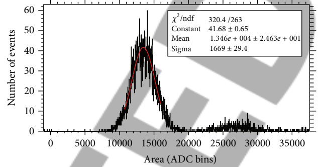
FIGURE 7: A sample fit of a tub signal.
