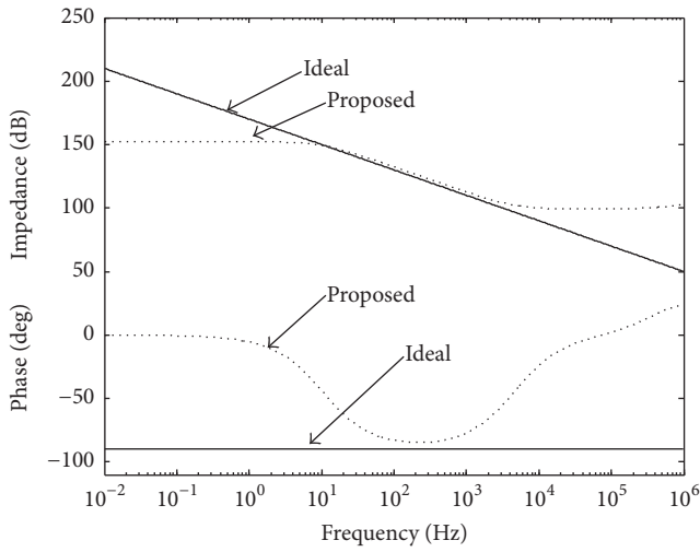
FIGURE 5: Compared impedance and phase for ideal and the proposed design.
