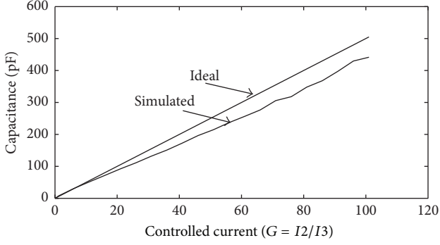
FIGURE 4: Plot of simulated capacitance and ideal case.
