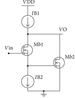
FIGURE 3: Circuit diagram for the buffer.
