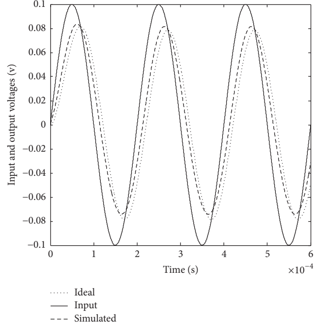
FIGURE 6: Simulation for the transient response.
