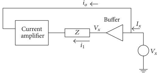
FIGURE 1: Block diagram of the proposed design.
