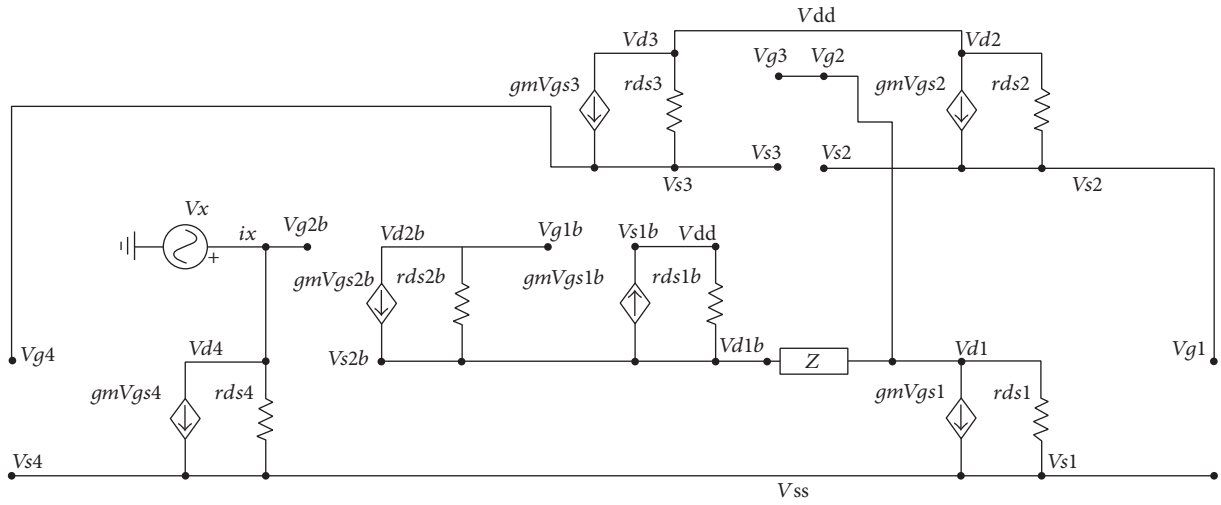
FIGURE 7: Small signal equivalent circuit of the proposed C-multiplier.
