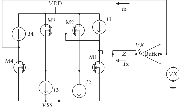
FIGURE 2: Circuit diagram of the proposed design.
