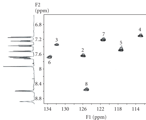
FIGURE 2: ^1\text{H}-^{13}\text{C} bidimensional heterocorrelated NMR spectrum of the compound [\text{Pd}(9\text{AA})(\mu\text{-Cl})]_2 (aromatic zone) where seven peaks of crossover are observed as indicator of the presence of a \sigma(\text{M}-\text{Csp}^2, \text{aryl}) bond.
