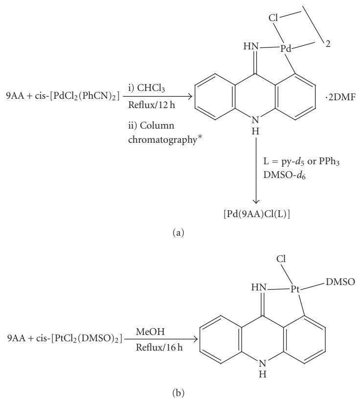
SCHEME 2: Scheme of the synthesis of the complexes (a) [\text{Pd}(9\text{AA})(\mu\text{-Cl})_2] and [\text{Pt}(9\text{AA})(\text{L})] (L = \text{py-}d_5 or \text{PPh}_3 ) and (b) [\text{Pt}(9\text{AA})\text{Cl}(\text{DMSO})] : *De SiO 2 . The eluted used was a mixture \text{CHCl}_3 :DMF (100:50).
