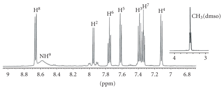
FIGURE 3: ^1\text{H} NMR spectrum of the complex [\text{Pt}(9\text{AA})\text{Cl}(\text{DMSO})] .
