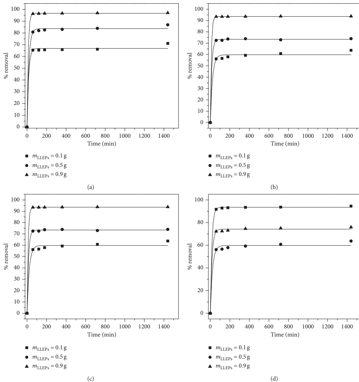
FIGURE 7: Effect of LLEPs dosage on the removal percentage of Pb(II) and Cd(II) in (a, b) monometal and (c, d) bimetal systems ( C_i = 100 mg/L; pH = 6).
