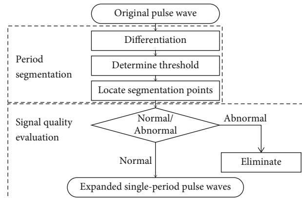
FIGURE 3: Steps of preprocessing. During period segmentation, the original pulse wave series were segmented into periods by threshold method. During signal quality evaluation, the segment obtained by period segmentation were divided into normal and abnormal segments by a logistic regression model. The abnormal segments were eliminated, and the range of normal segment was expanded by 50% on both sides to include the information of adjacent periods.
