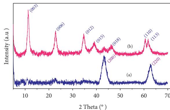
FIGURE 3: X-ray diffraction powder patterns of (a) HT3-MW-Ec and (b) HT3-W-EcR.
