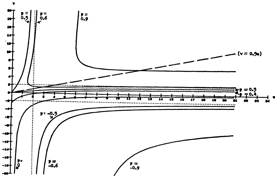
Figure 1: Curves along which (u, v) may be placed to change the value of the correlation coefficient to selected values p for r = b = 0.5 and n = 12 .
