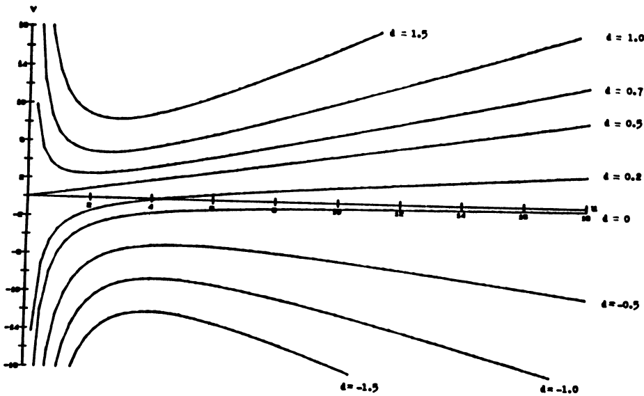
Figure 2: Curves along which (u, v) may be placed to change the value of the slope to selected values d for r = b = 0.5 and n = 12 .
