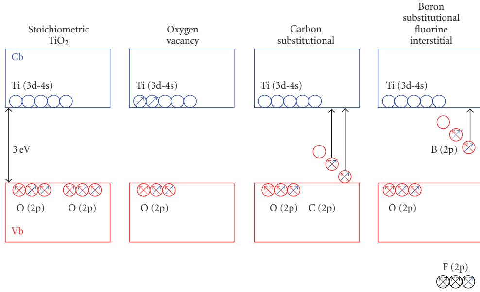
FIGURE 3: Schematic representation of the electronic structure. (a) Far left: TiO 2 , (b) left center: with oxygen vacancy, (c) right center: with carbon doping, (d) far right: with B and F codoping. The valence band is principally oxygen 2p in character. The conduction band is principally Ti 3d & 4s in character. In the atomic limit, each TiO 2 unit contributes two filled oxygen 2p orbitals, four half-filled oxygen 2p orbitals, and four titanium valence electrons. In the pure material, (far left) the four titanium valence electrons fill the vacant oxygen 2p orbitals. When an oxygen atom is removed, (center left) three oxygen 2p orbitals are removed, but only 4 electrons. The remaining two electrons are forced to reside in Ti 3d orbitals. Upon substitution of C for O, (center right) the carbon 2p bands “float up” into the band gap due to weaker nuclear-electron interaction. Onsets in the photoabsorption spectrum are seen corresponding to transitions from both occupied carbon 2p bands to the conduction band. B-F codoping (far right) fills the half-full F-2p orbital with a large energy benefit.
