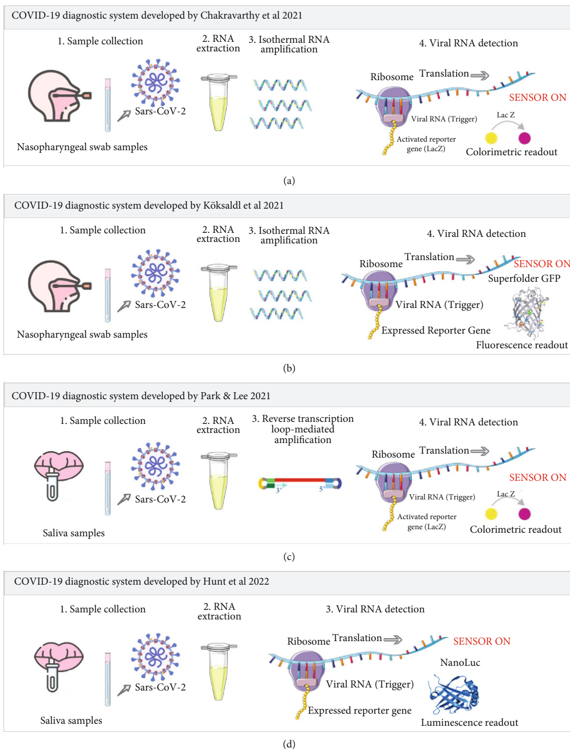
FIGURE 2: General scheme of the currently developed toehold switch-based diagnostics for COVID-19: (a) a system developed by Chakravarthy et al. [40] which utilized NASBA (nucleic acid sequence-based amplification) for amplifying trigger RNA from patient's nasopharyngeal swab sample and toehold switch-based biosensor with lacZ as a reporter gene, (b) a system developed by Köksaldı et al. [41] which utilized NASBA for amplifying trigger RNA from patient's nasopharyngeal swab sample and toehold switch-based biosensor with superfolder GFP as a reporter gene, (c) a system developed by Park et al. [42] which utilized reverse transcription loop-mediated amplification (RT-LAMP) for amplifying trigger RNA from patient's saliva sample and toehold switch-based biosensor with lacZ as a reporter gene, and (d) a trigger RNA amplification-free system developed by Hunt et al. [43] which detected SARS-CoV-2 RNA from patient's saliva sample using toehold switch-based biosensor with NanoLuc as a reporter gene.
