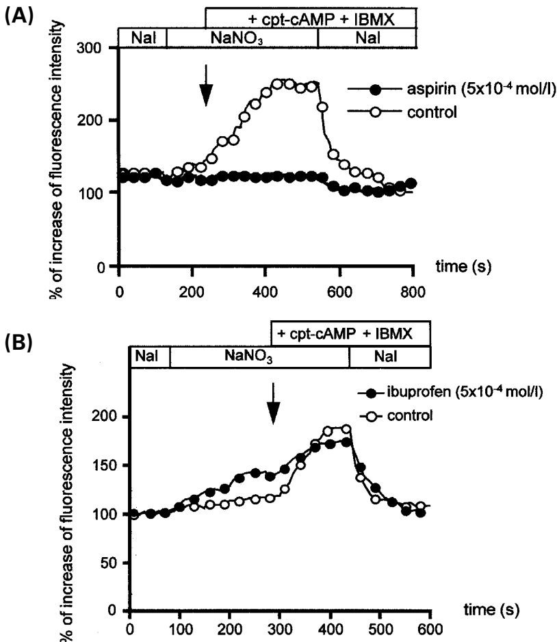
FIG. 7. The fluorescence of intracellular MEQ was measured with respect to time under control conditions and after 48 h of treatment with either 5x10 -4 mol/l aspirin (A) or 5x10 -4 mol/l ibuprofen (B). The sequence of buffer substitutions is indicated in the inset.
