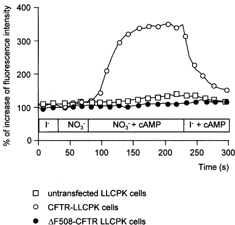
FIG. 2. Validation of the MEQ technology. The fluorescence of intracellular MEQ was registered in untransfected LLCPC cells ( \square ) and in LLCPC cells expressing either the wild type CFTR ( \circ ) or the \Delta F_{508} -CFTR ( \bullet ), under sequential anionic substitutions of the superfusing medium and addition of permeant cpt-cAMP, as indicated in the inset and described in materials and methods.
