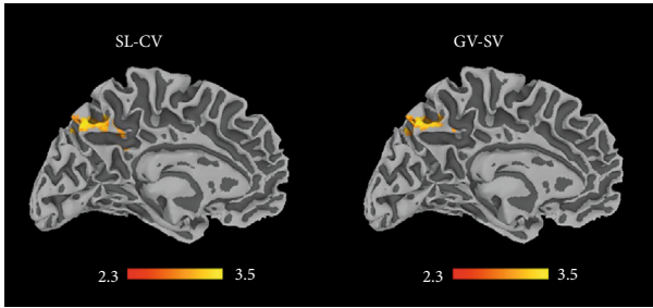
FIGURE 4: Neuroimaging-behavioral correlations, in particular correlations of brain activity during AO of gait and (a) SL-CV or (b) GV-SV. The results are cluster corrected for multiple comparisons ( Z \geq 2.3 , p < 0.05 ) and are shown in MNI space.
