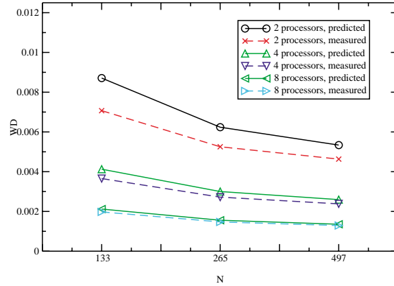
Fig. 19. Measured versus predicted work distribution values of HNS for CYCLIC distribution and various problem ( N ) and machine sizes.
